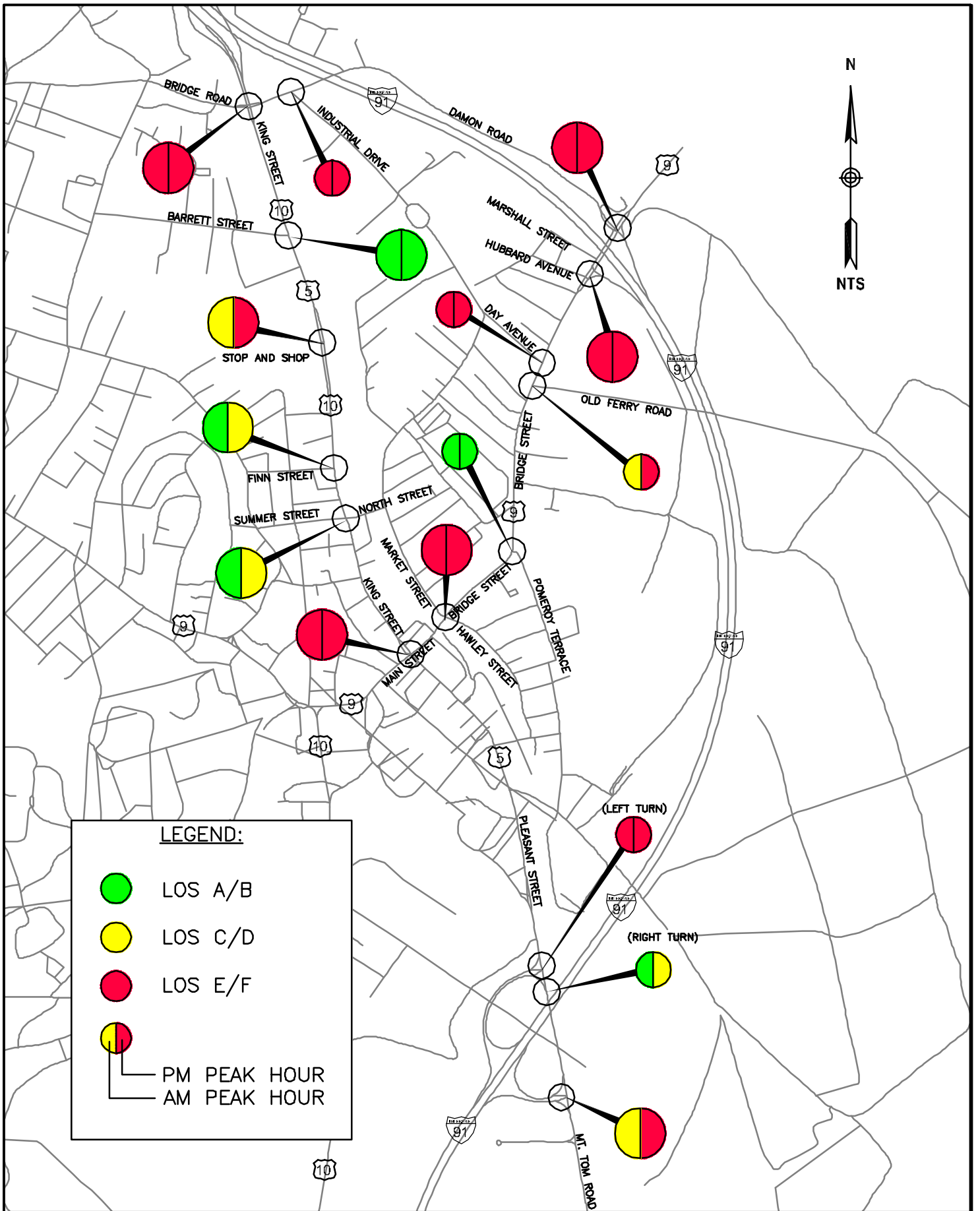
Figure 5 2009 Existing LOS Summary I-91 Interchange 19 Project Northampton, MA
