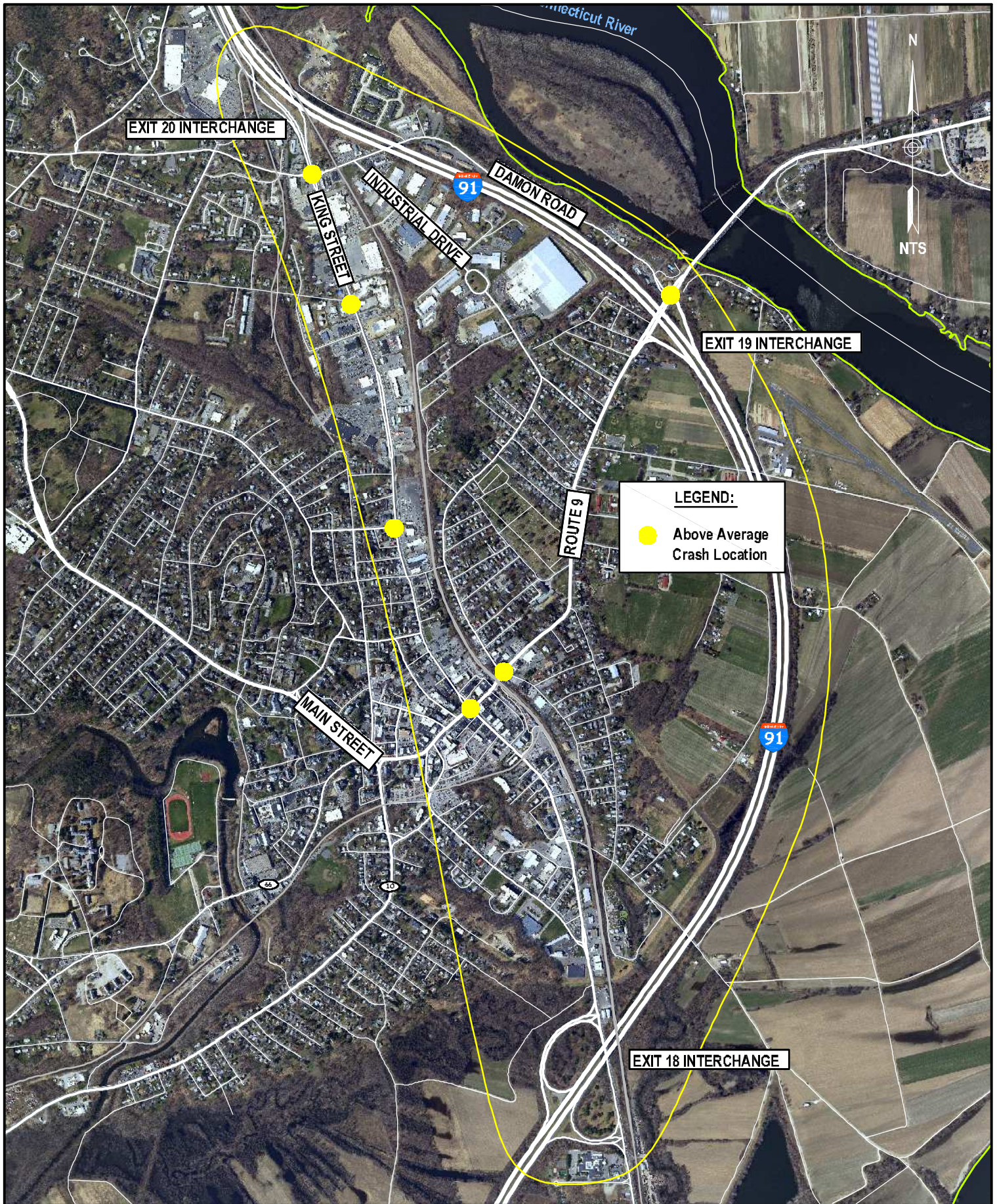
Figure 6 Above Average Crash Locations I-91 Interchange 19 Project Northampton, MA
